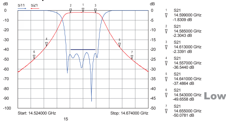
Real diplexer's behaviour
